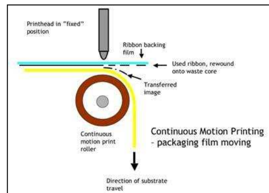
Continuous Motion TTO
