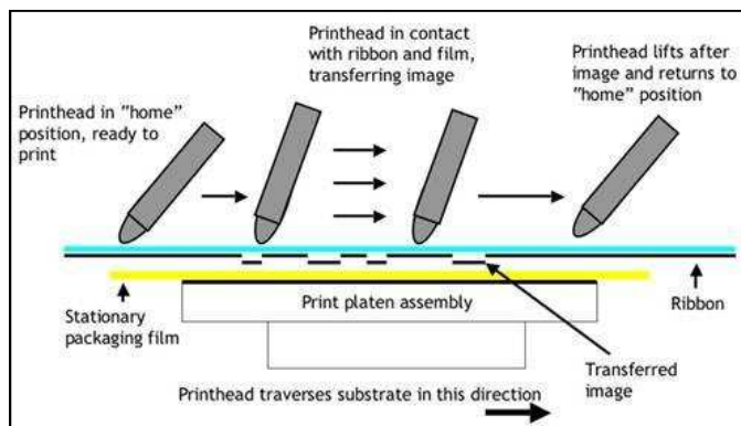
Intermittent Motion TTO
